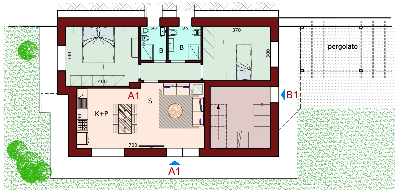
PIANO TERRA
